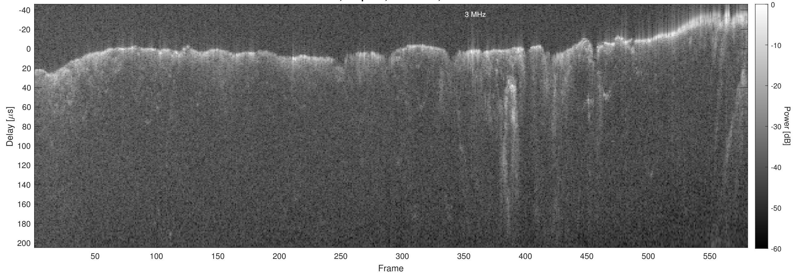
Orbit 4768, Chapman, No Window, Channel 2
