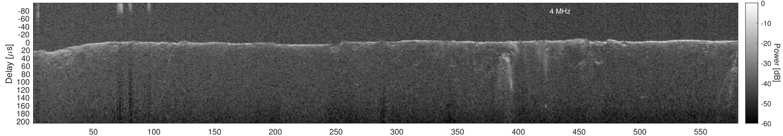
Orbit 4768, Cluttergram
