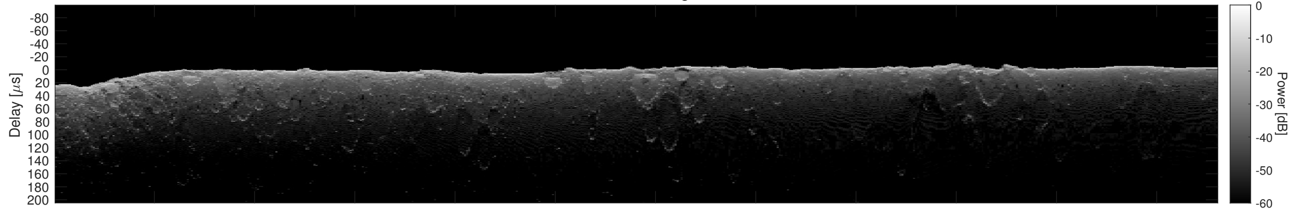
Orbit 4768, Cluttergram
