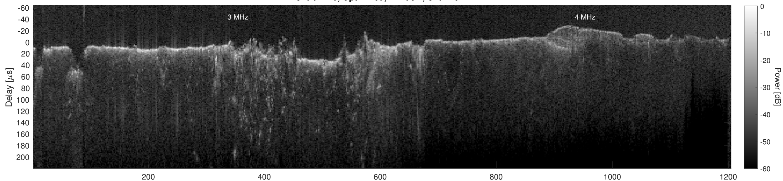
Orbit 4770, Cluttergram
