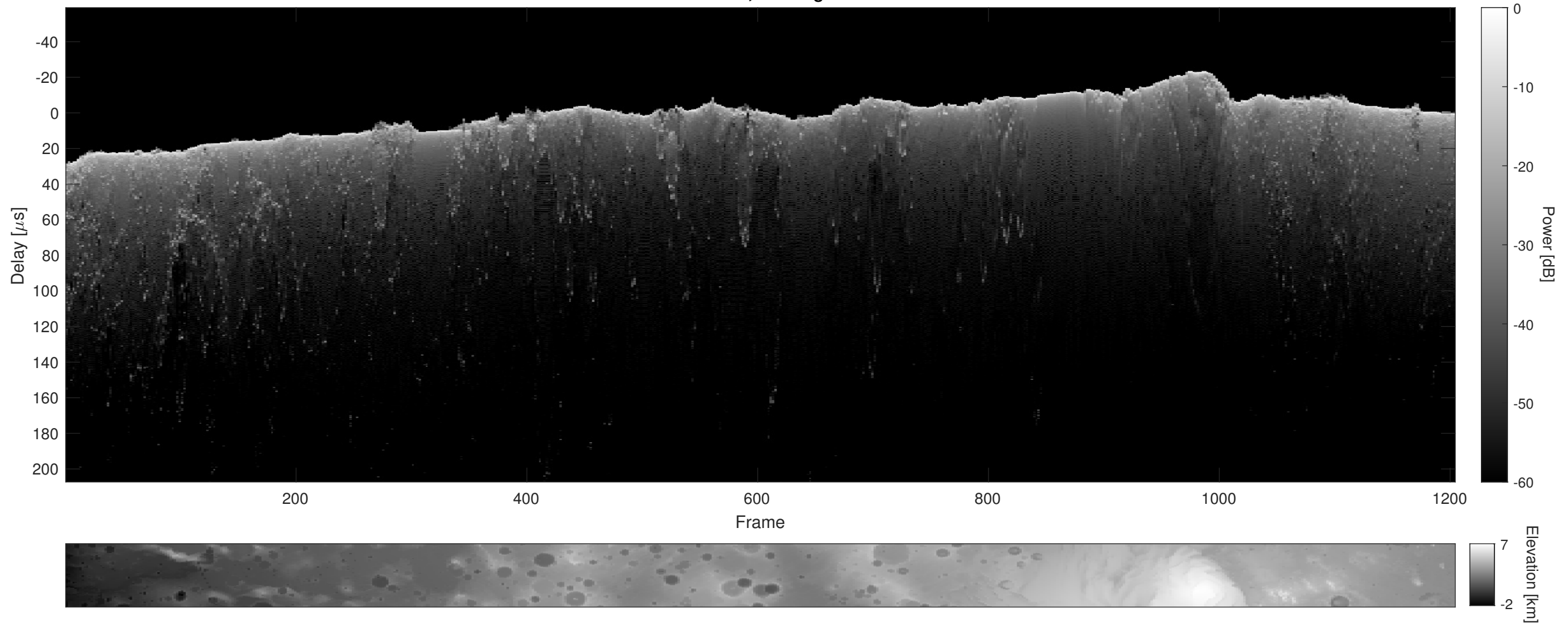
Orbit 4771, Cluttergram
