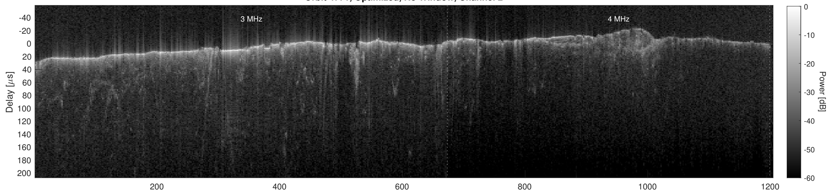
Orbit 4771, Cluttergram
