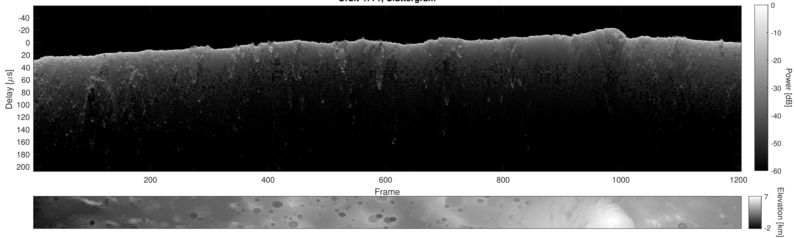
Orbit 4771, Cluttergram
