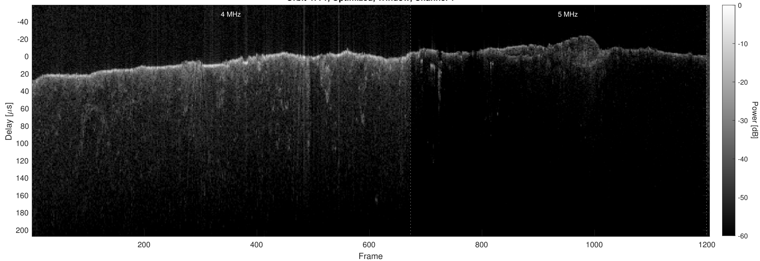
Orbit 4771, Optimized, Window, Channel 2
