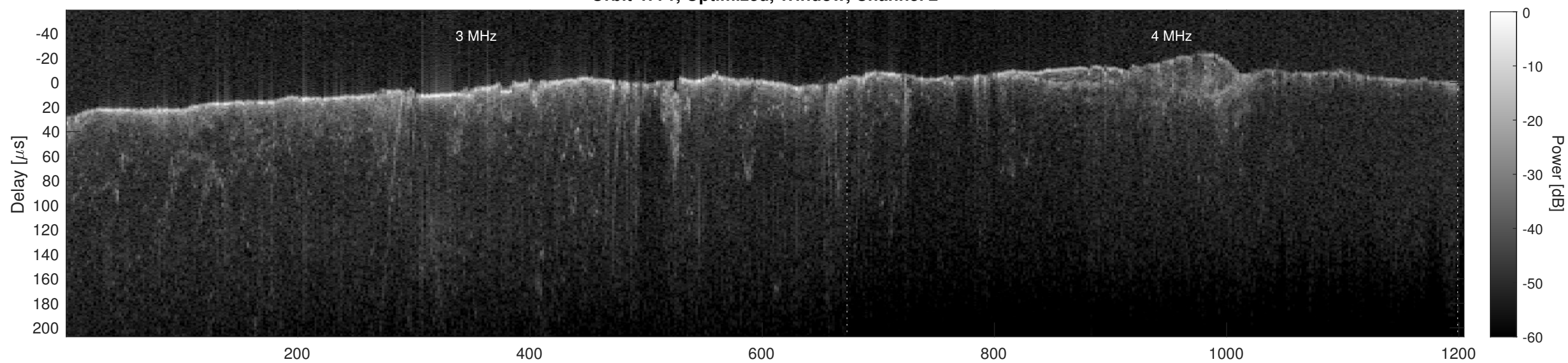
Orbit 4771, Cluttergram
