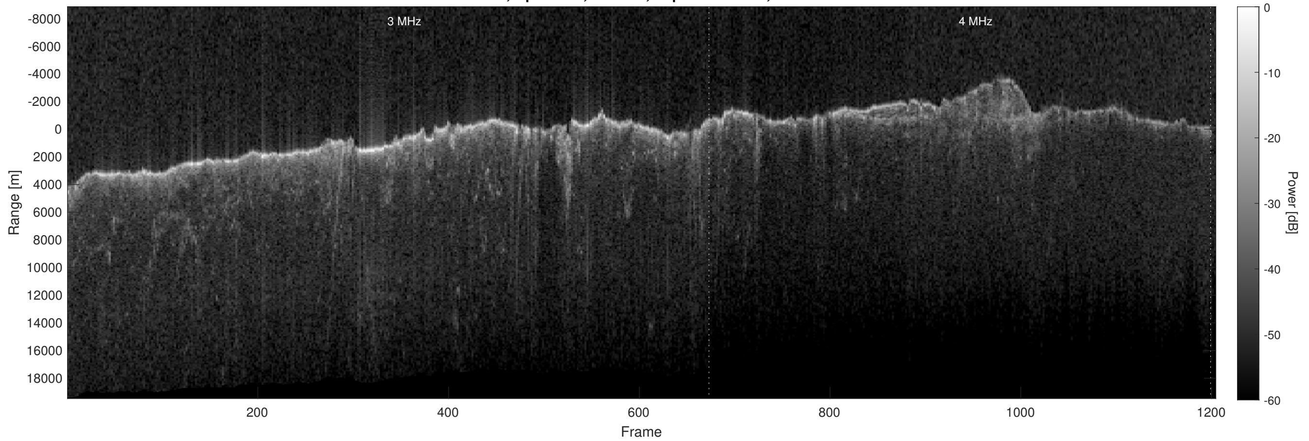
Orbit 4771, Optimized, Window, Depth-Corrected, Channel 2
