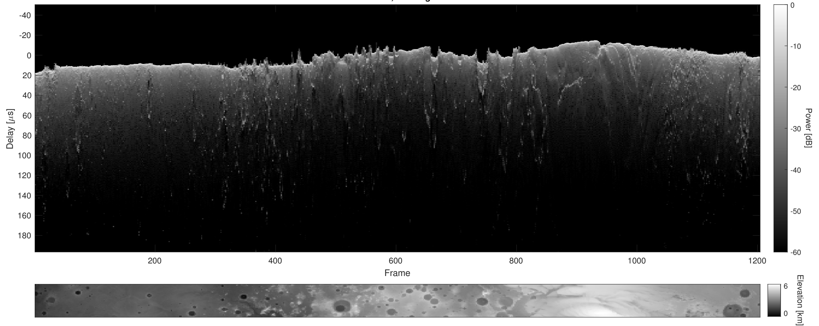
Orbit 4772, Cluttergram
