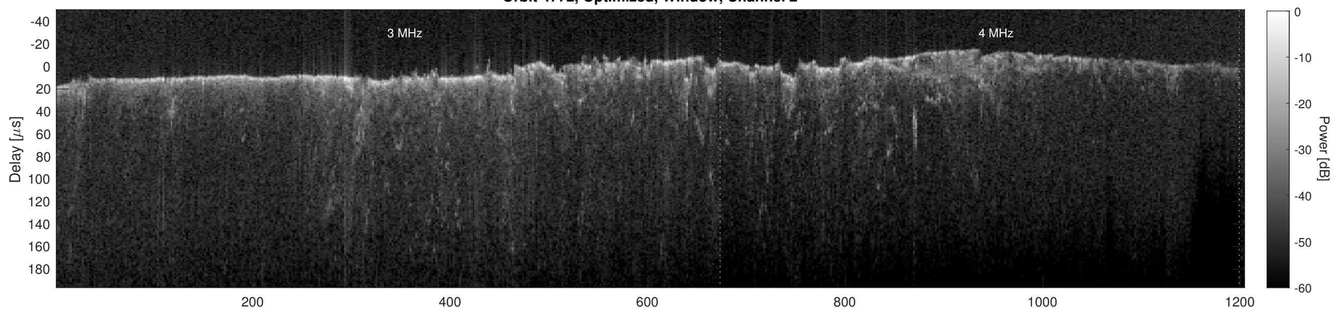
Orbit 4772, Cluttergram
