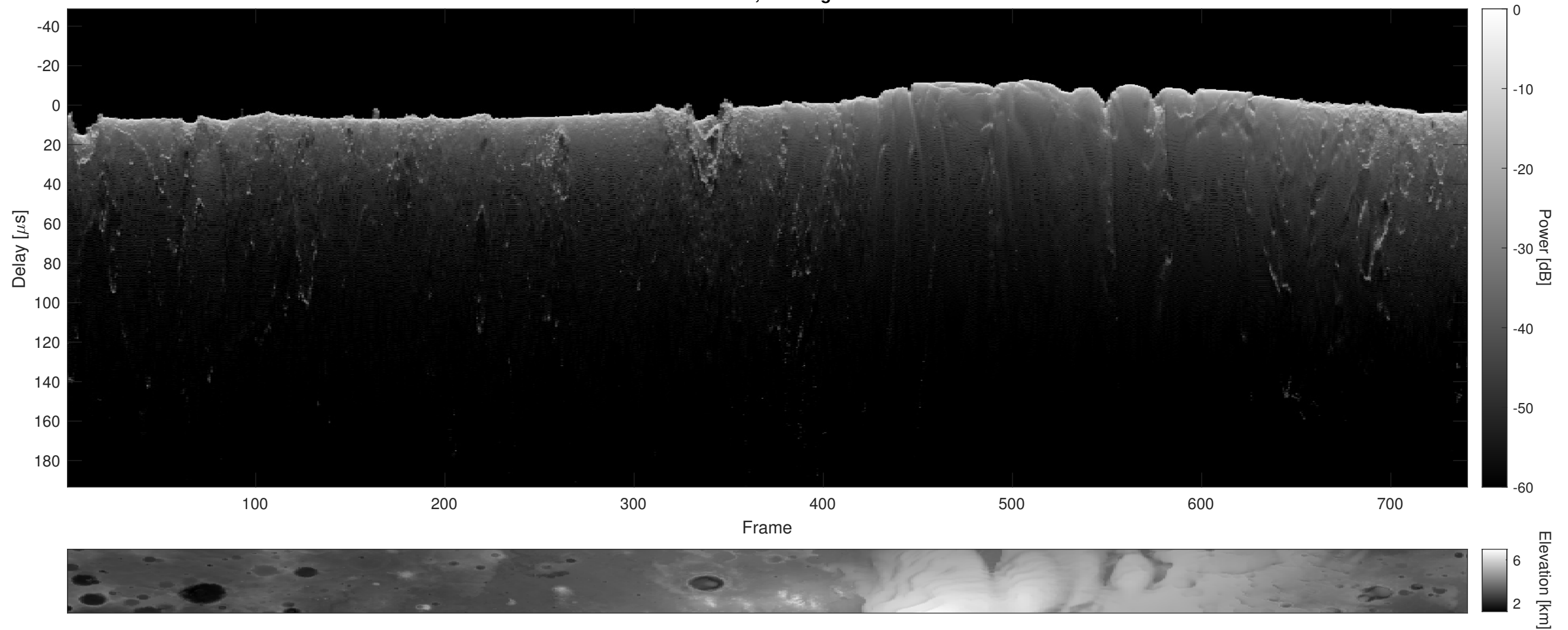
Orbit 4773, Cluttergram
