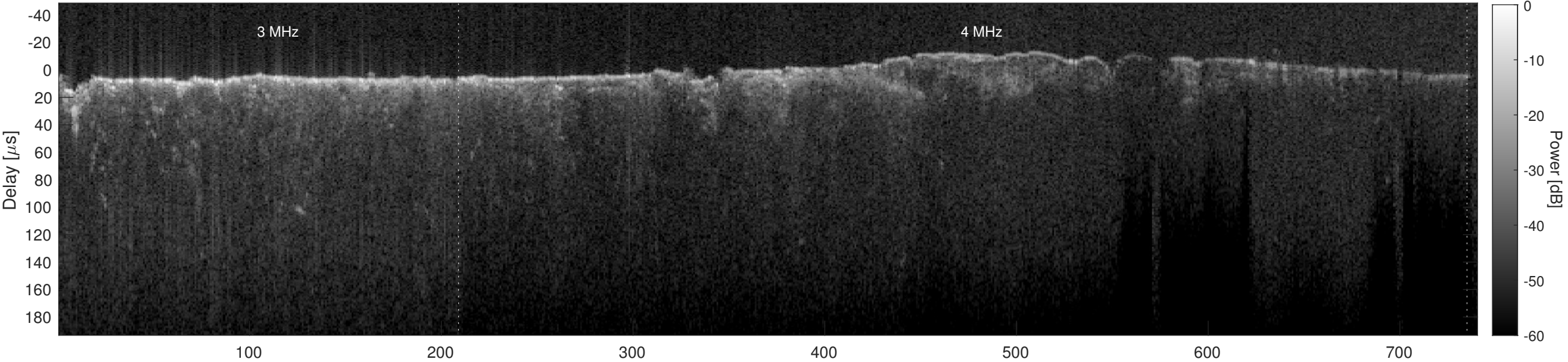
Orbit 4773, Cluttergram
