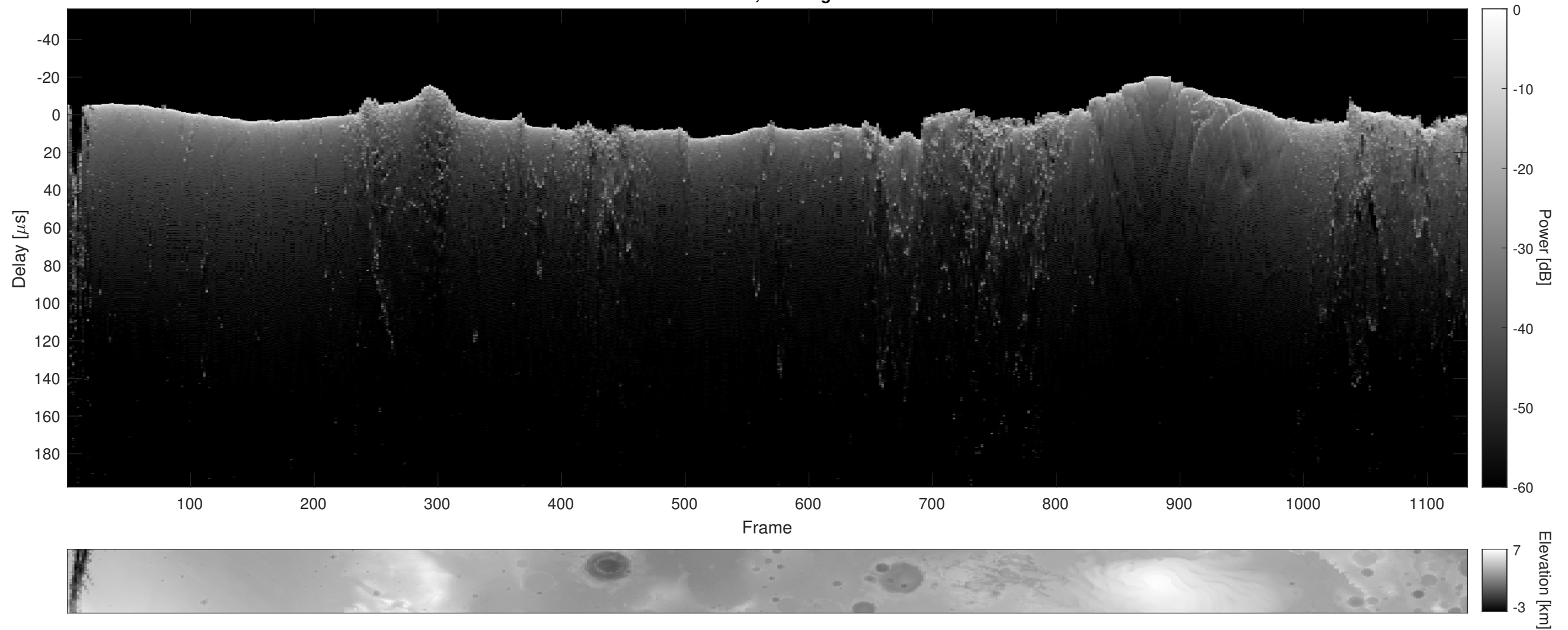
Orbit 4774, Cluttergram
