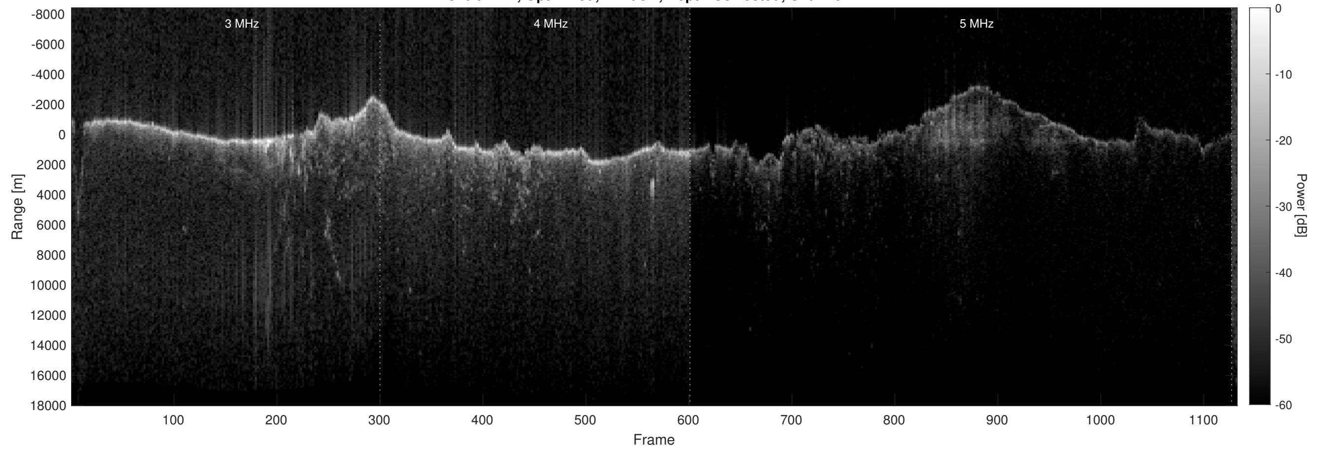
Orbit 4774, Optimized, Window, Depth-Corrected, Channel 2
