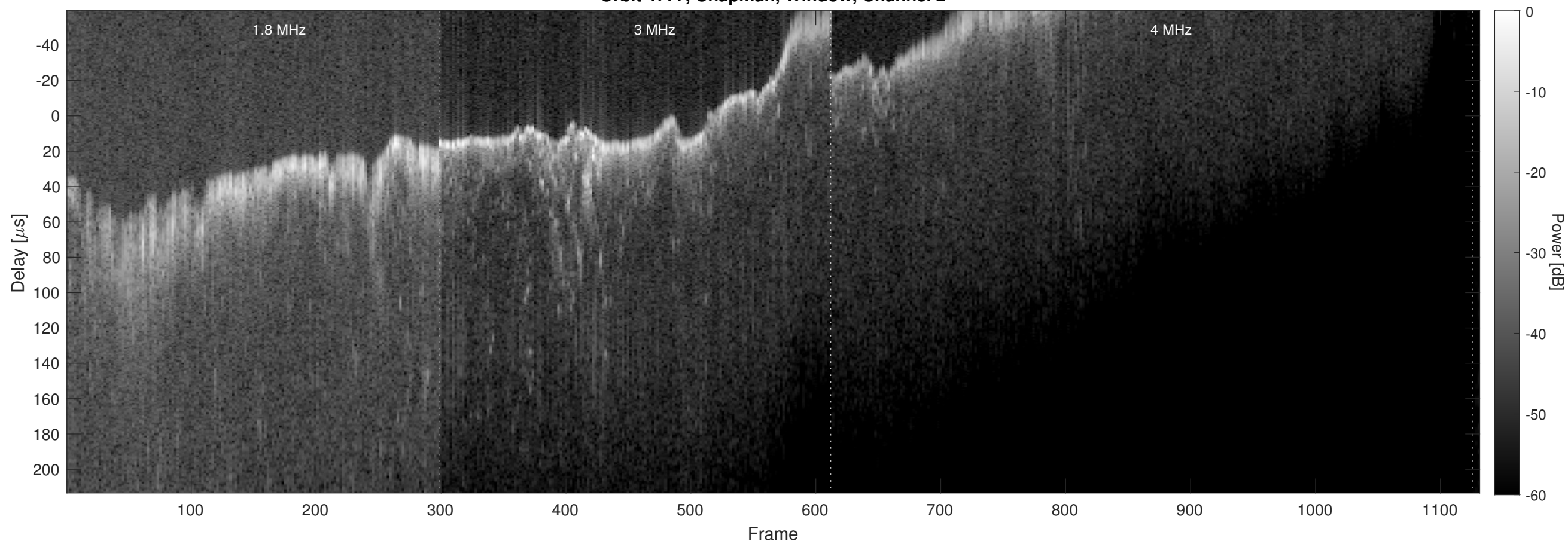
Orbit 4777, Chapman, Window, Channel 2
