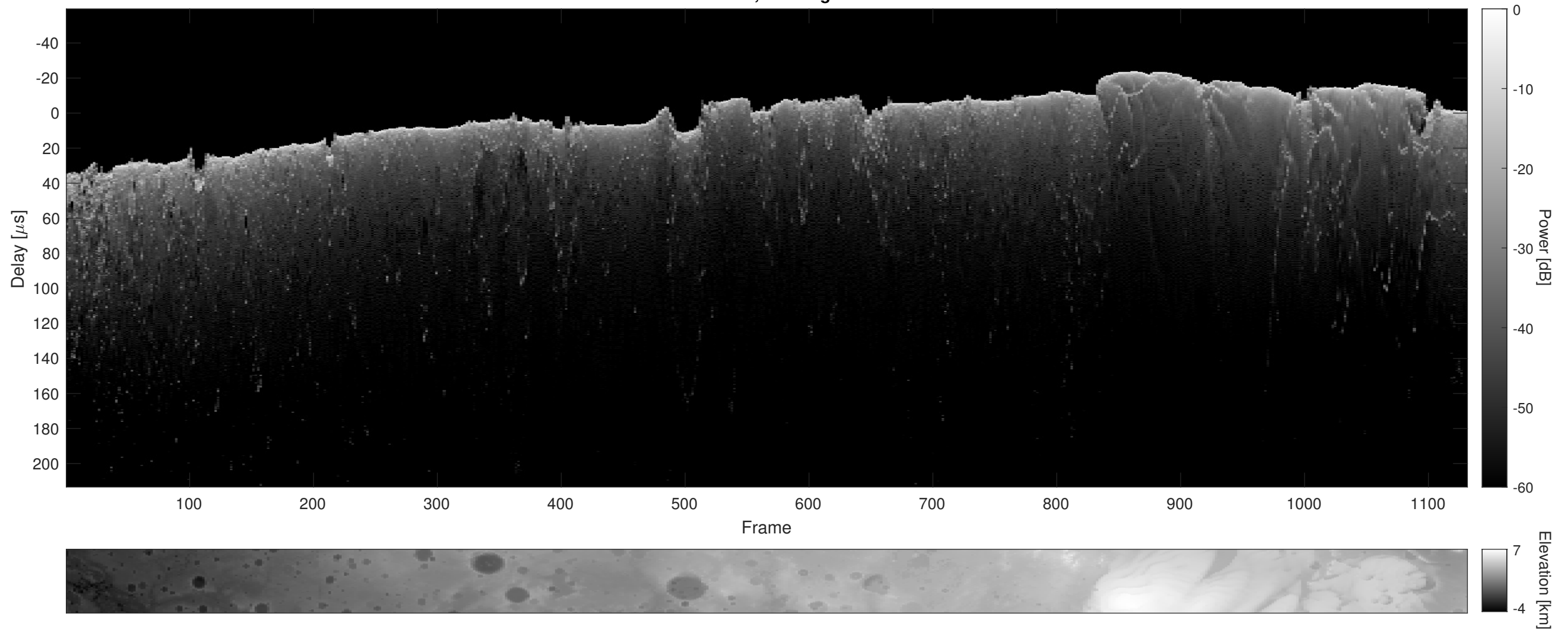
Orbit 4777, Cluttergram
