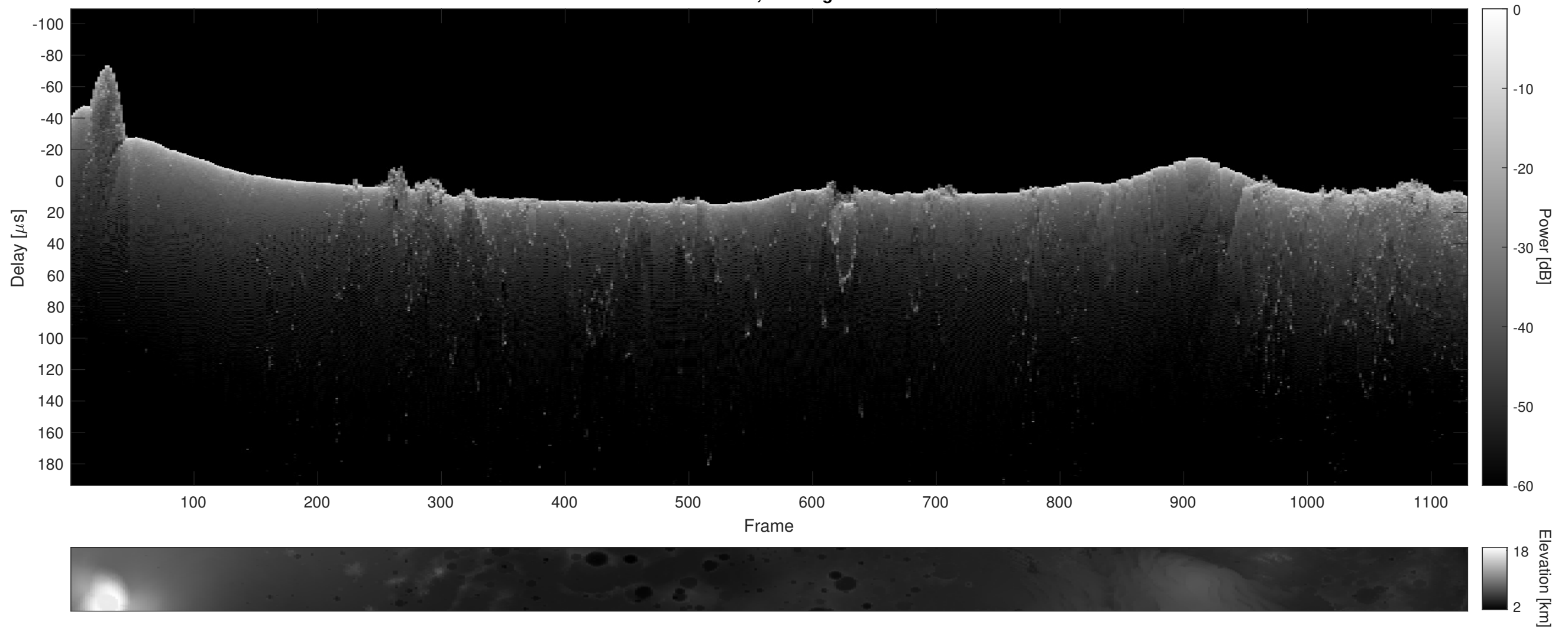
Orbit 4778, Cluttergram
