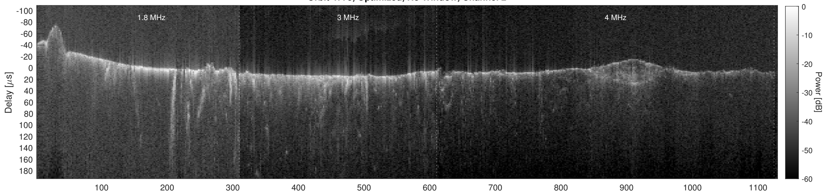
Orbit 4778, Cluttergram
