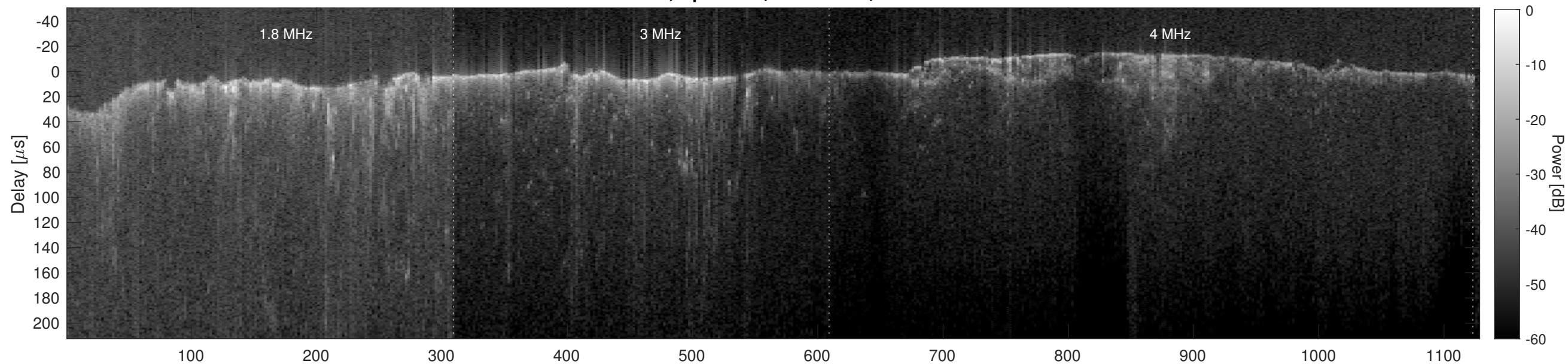
Orbit 4779, Cluttergram
