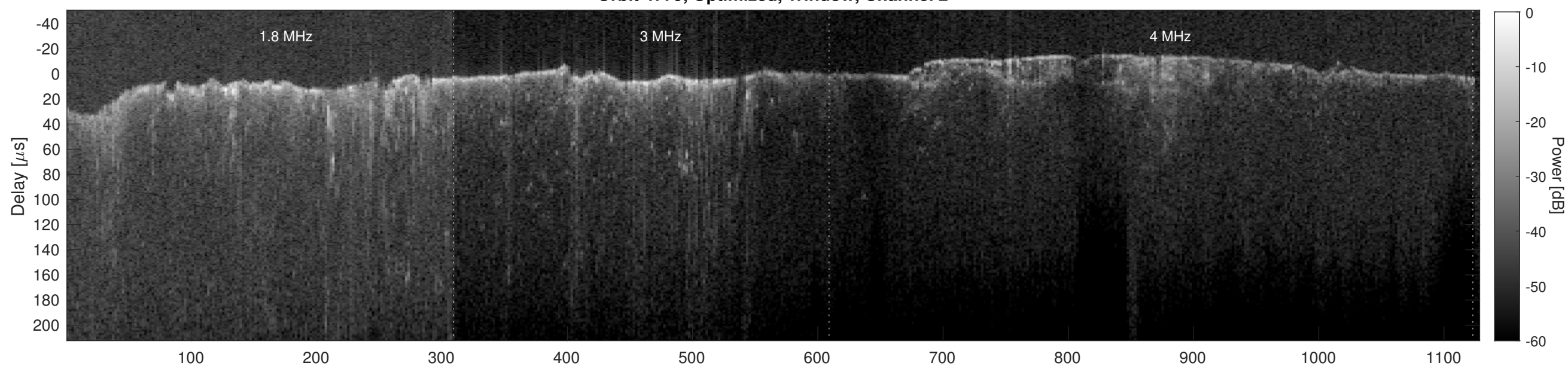
Orbit 4779, Cluttergram
