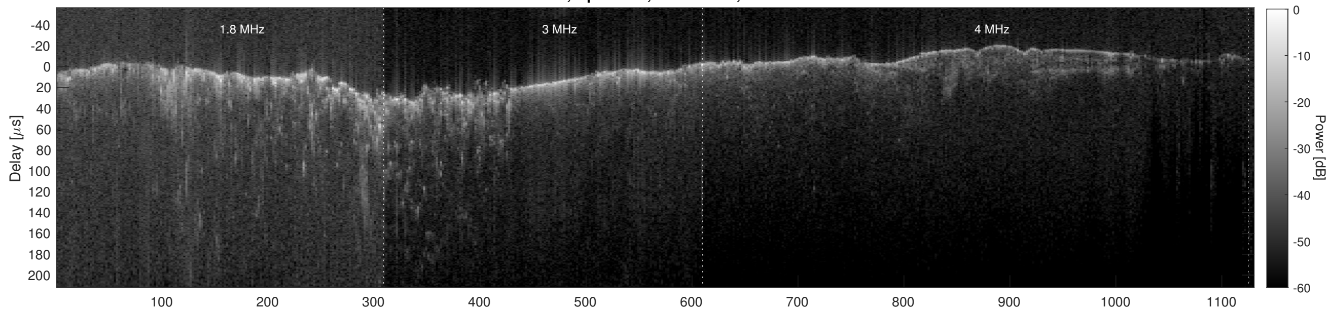
Orbit 4780, Cluttergram
