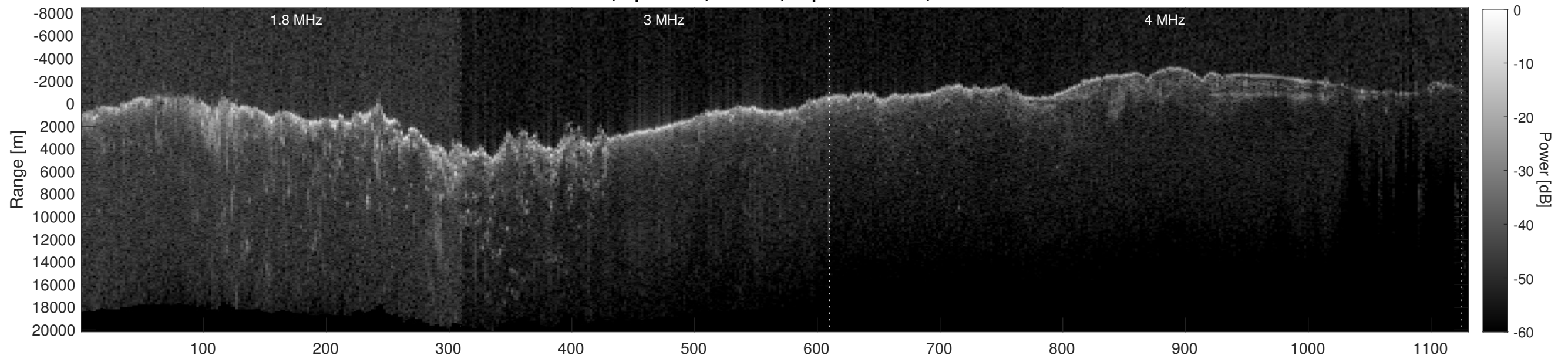
Orbit 4780, Depth-Corrected Cluttergram
