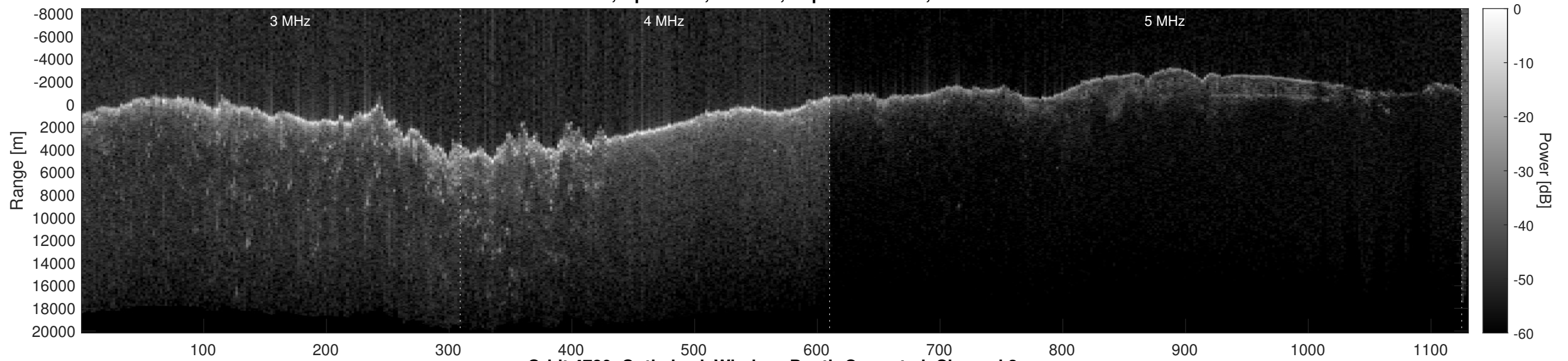
Orbit 4780, Optimized, Window, Depth-Corrected, Channel 2
