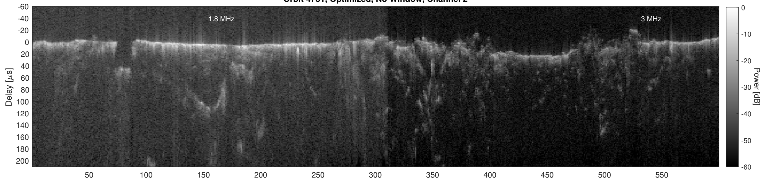
Orbit 4781, Cluttergram
