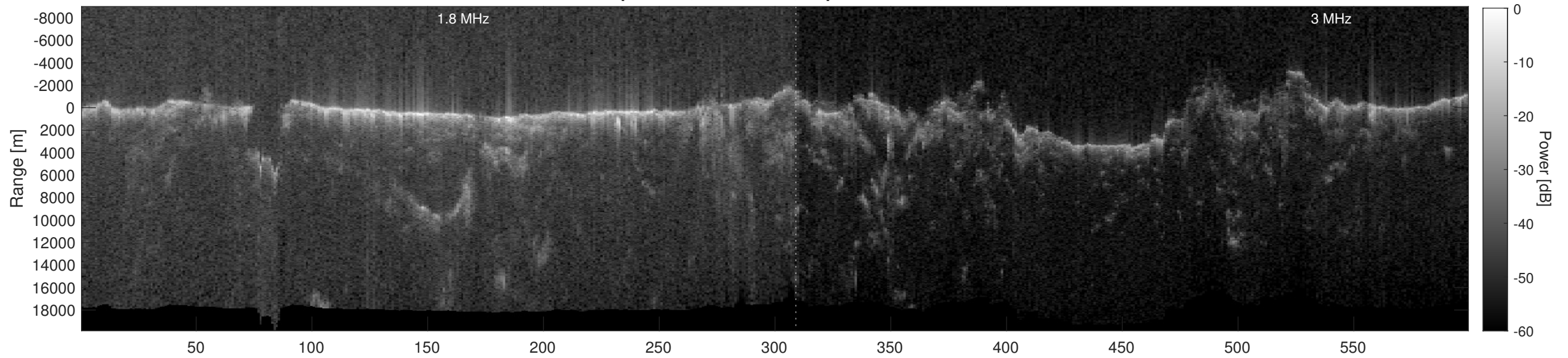
Orbit 4781, Depth-Corrected Cluttergram
