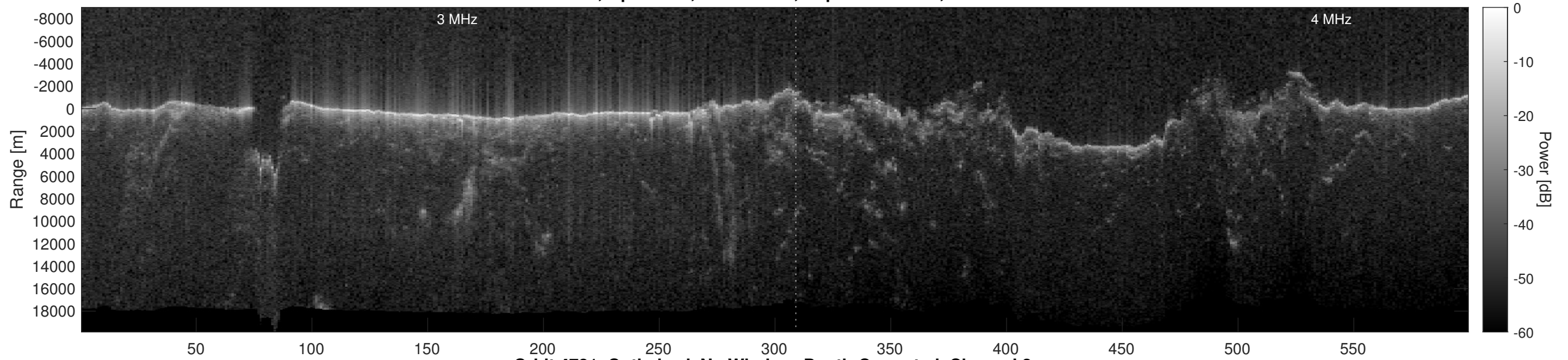
Orbit 4781, Optimized, No Window, Depth-Corrected, Channel 2
