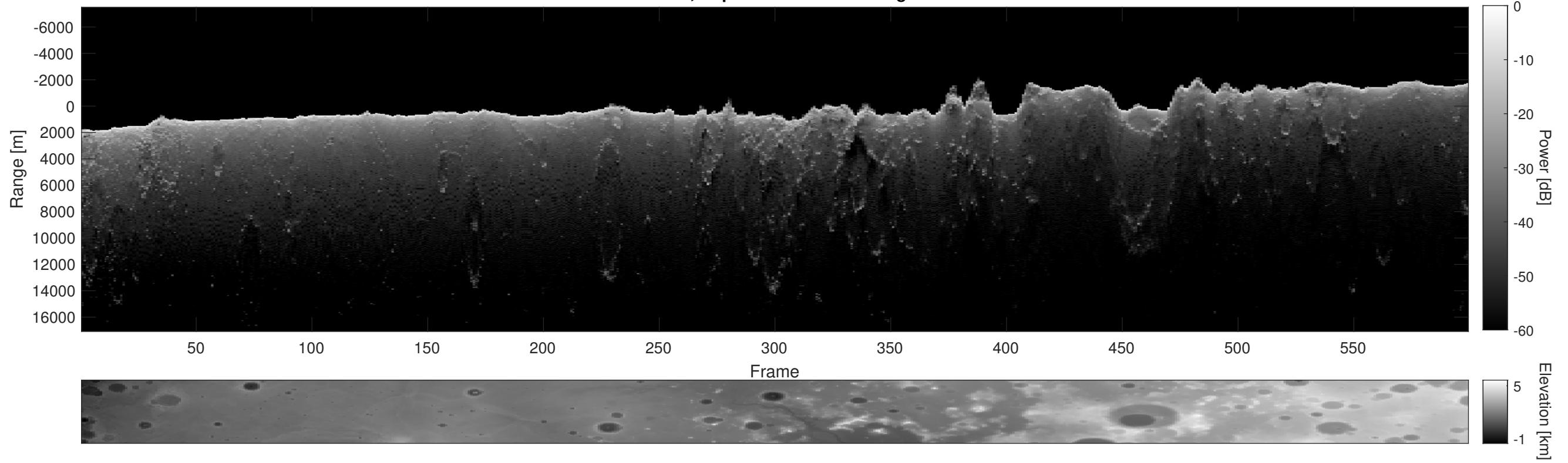
Orbit 4783, Depth-Corrected Cluttergram
