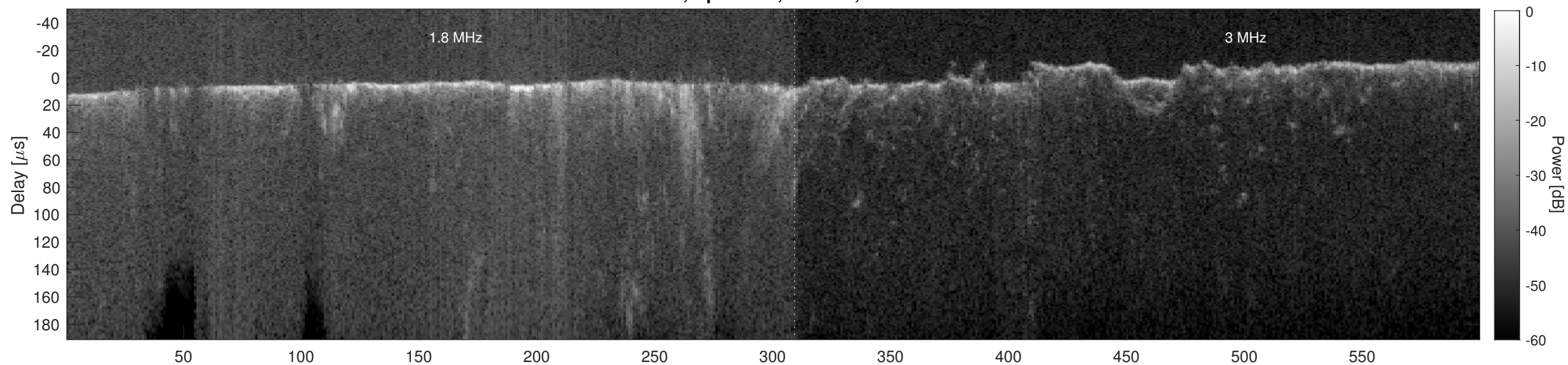
Orbit 4783, Cluttergram
