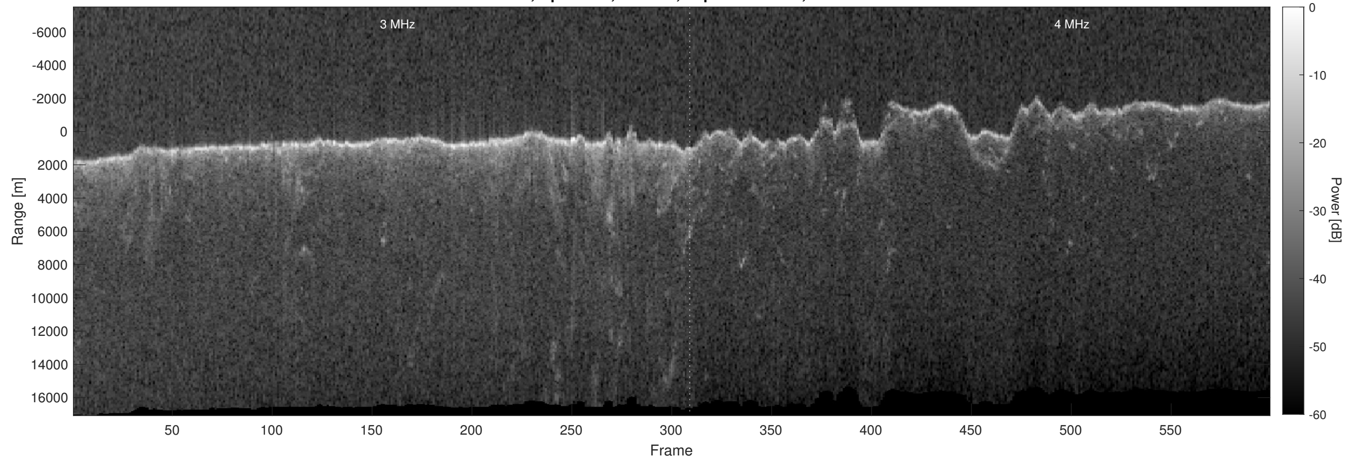
Orbit 4783, Optimized, Window, Depth-Corrected, Channel 2
