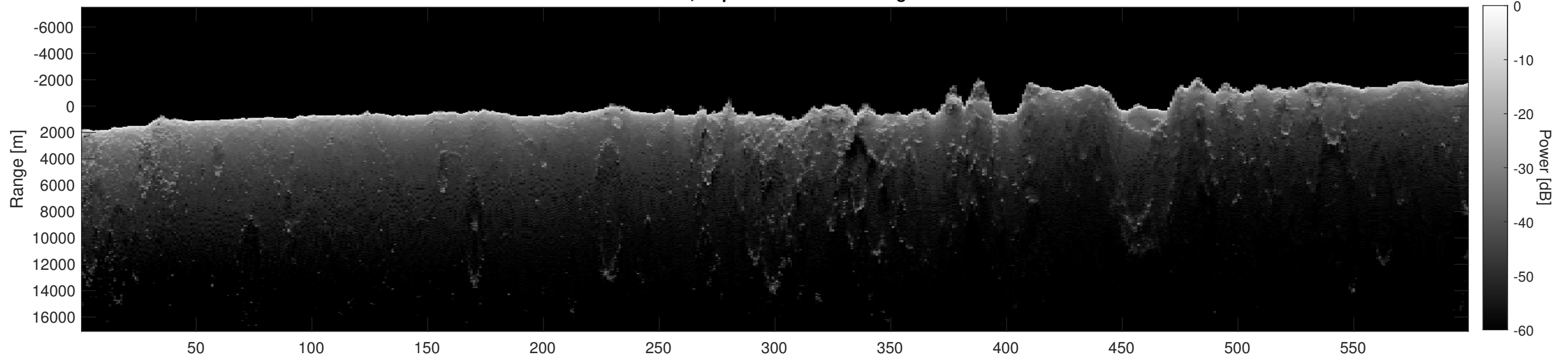
Orbit 4783, Depth-Corrected Cluttergram
