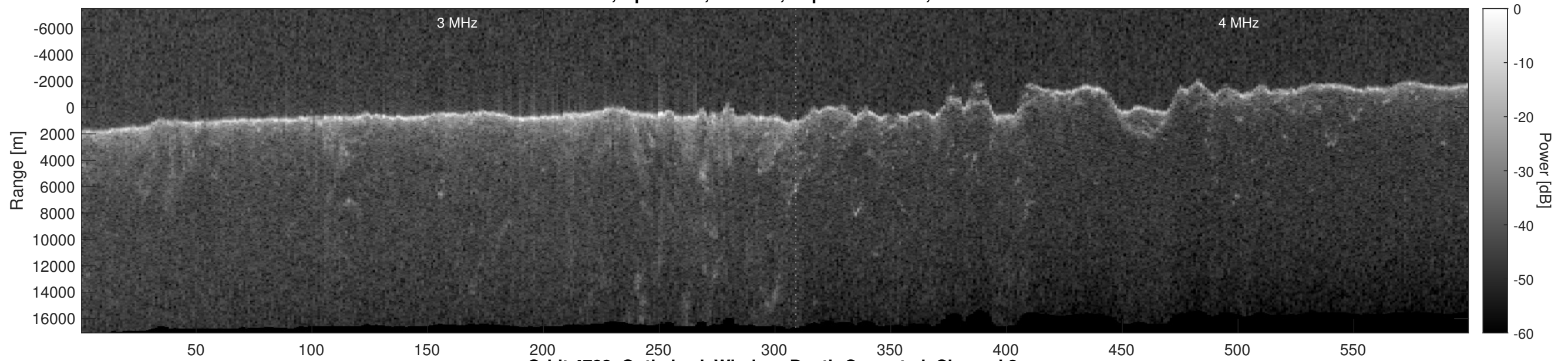
Orbit 4783, Optimized, Window, Depth-Corrected, Channel 2
