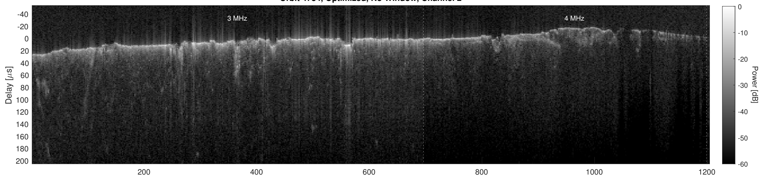
Orbit 4784, Cluttergram
