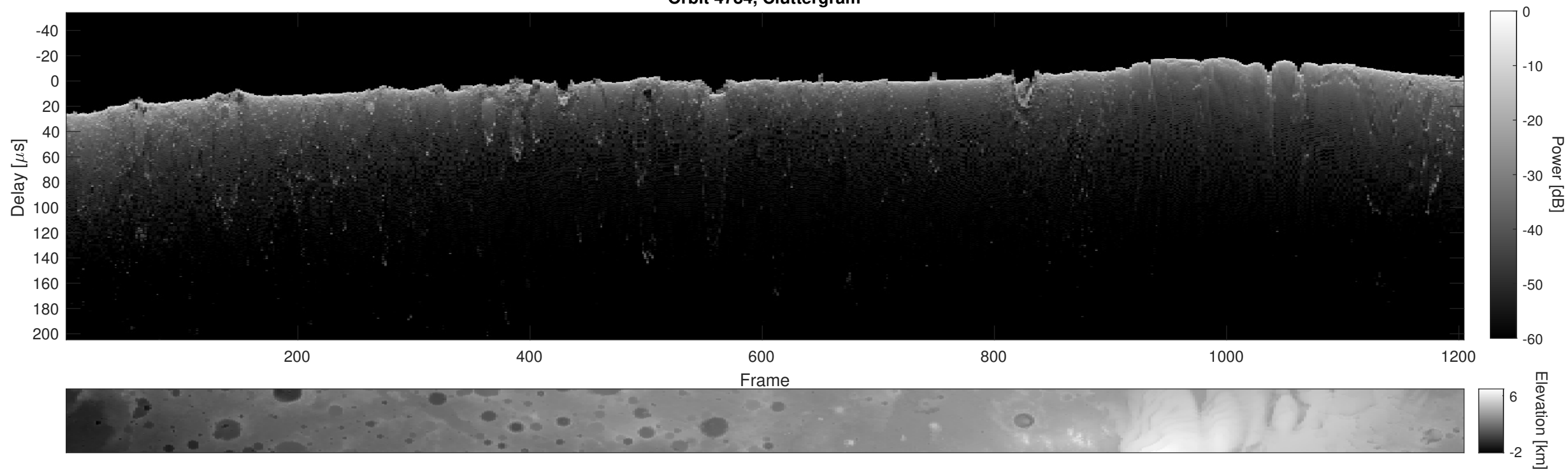
Orbit 4784, Cluttergram
