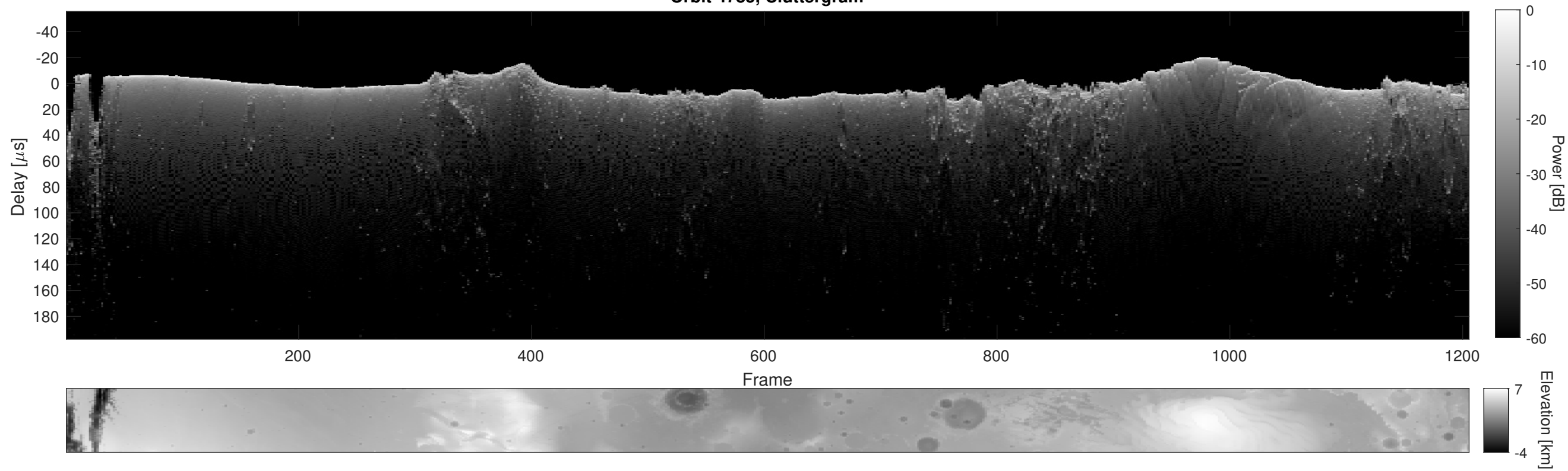
Orbit 4785, Cluttergram
