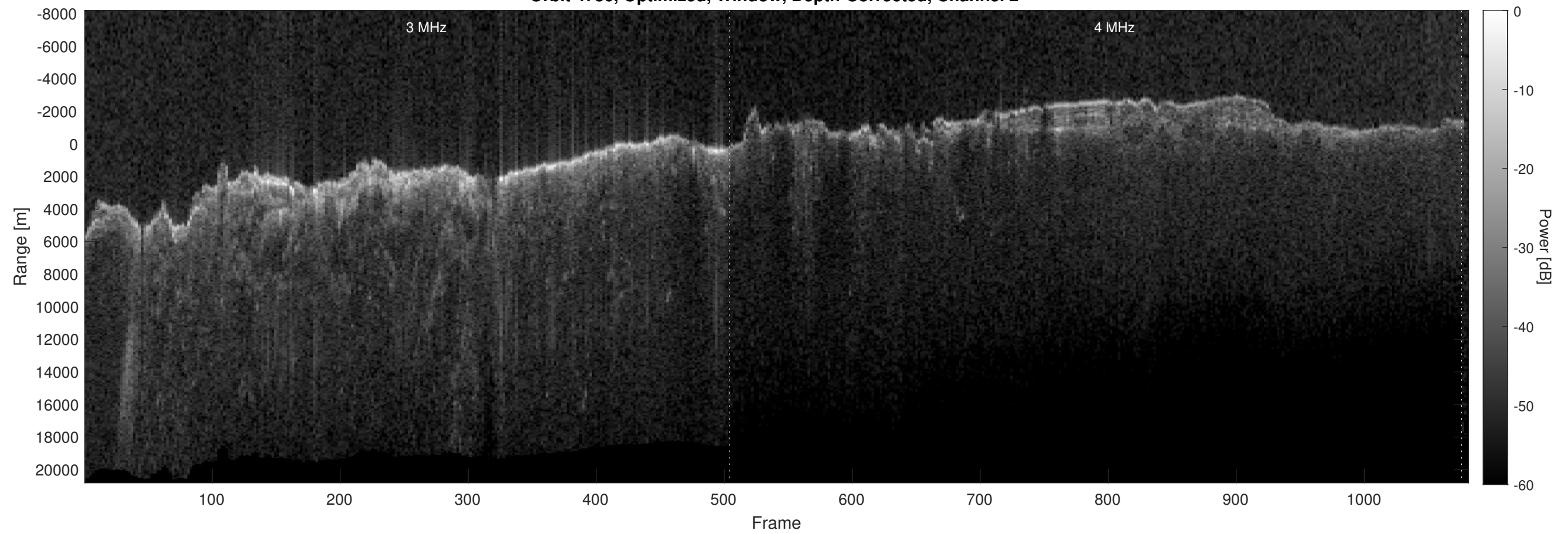
Orbit 4786, Optimized, Window, Depth-Corrected, Channel 2
