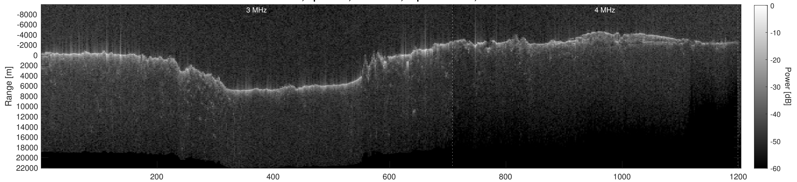
Orbit 4787, Depth-Corrected Cluttergram
