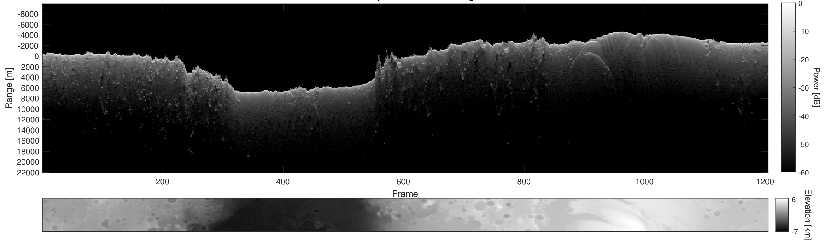
Orbit 4787, Depth-Corrected Cluttergram
