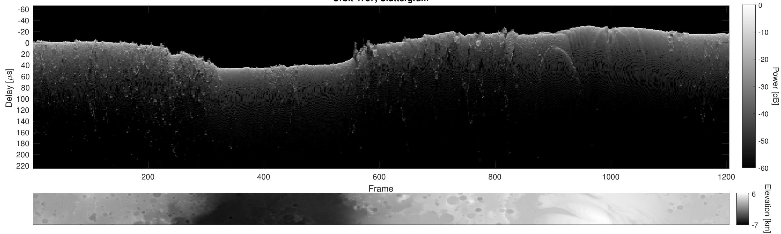
Orbit 4787, Cluttergram
