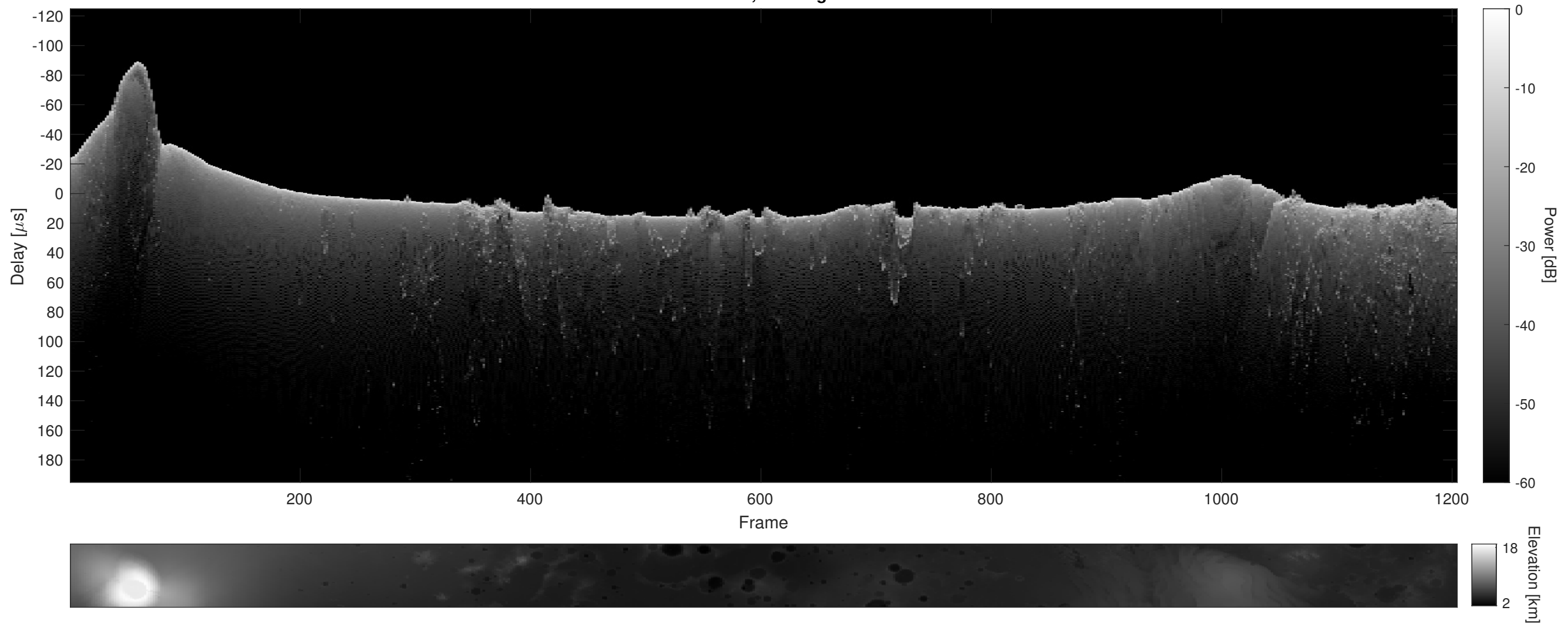
Orbit 4789, Cluttergram
