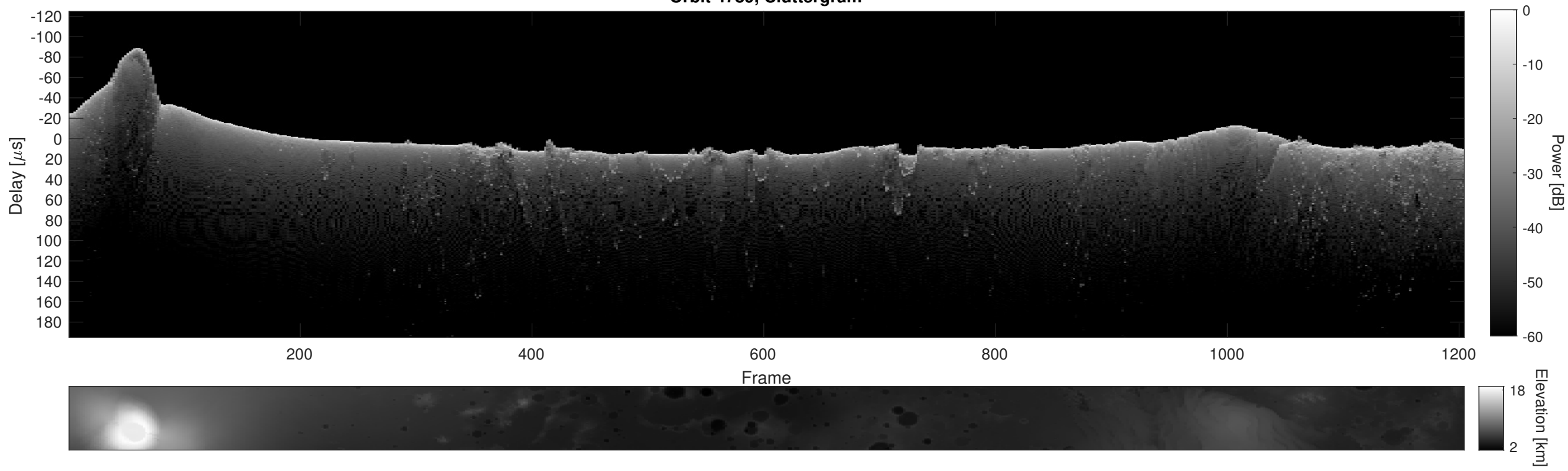
Orbit 4789, Cluttergram
