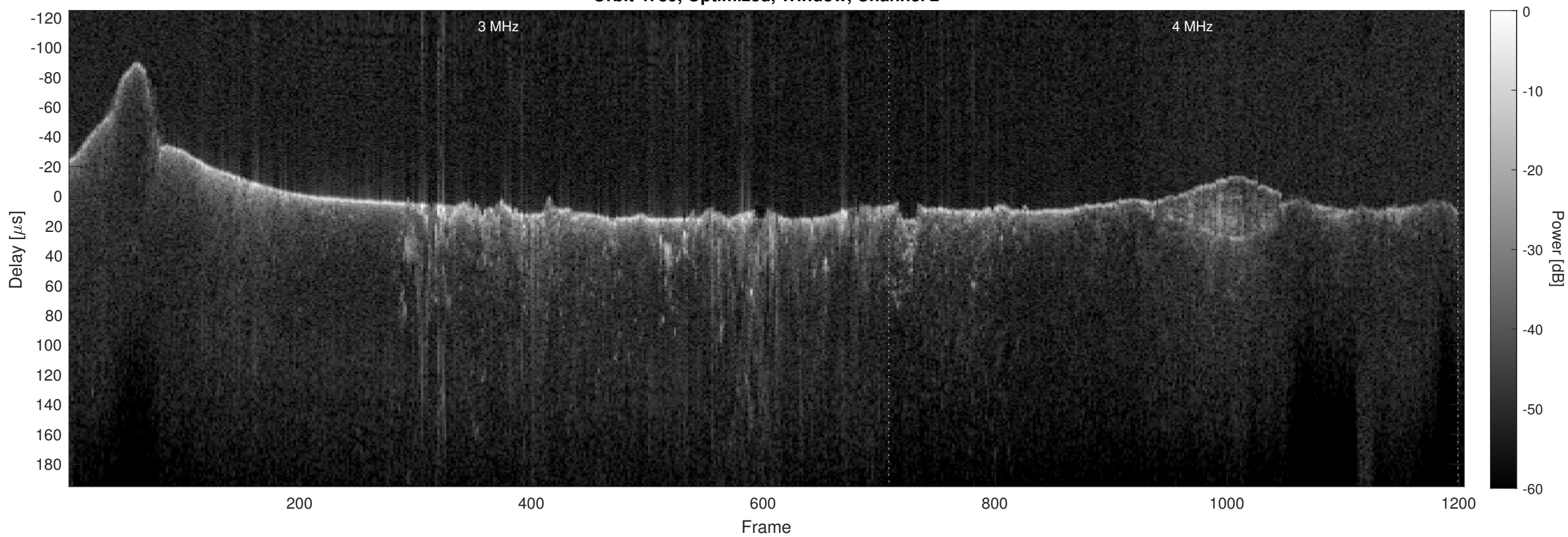
Orbit 4789, Optimized, Window, Channel 2
