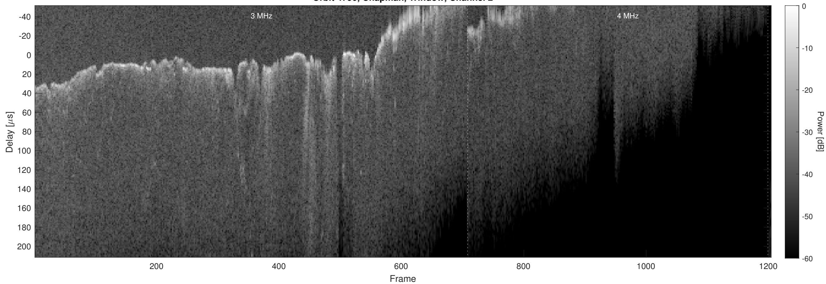
Orbit 4790, Chapman, Window, Channel 2
