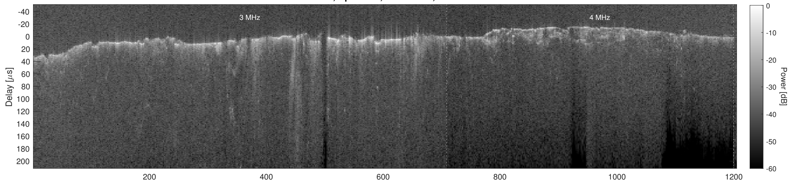
Orbit 4790, Cluttergram
