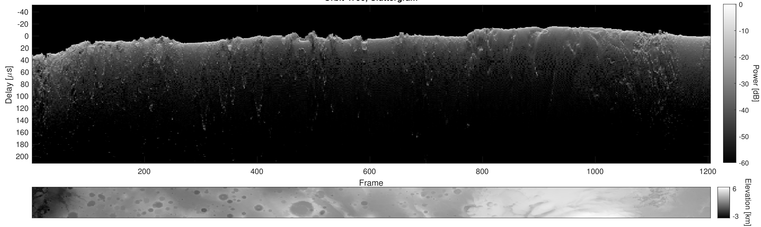
Orbit 4790, Cluttergram
