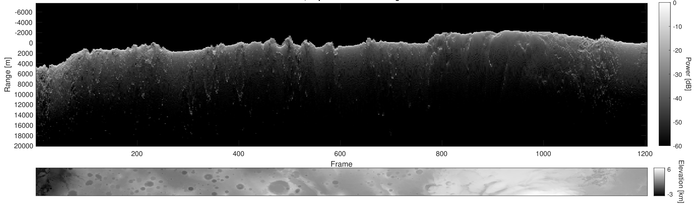
Orbit 4790, Depth-Corrected Cluttergram
