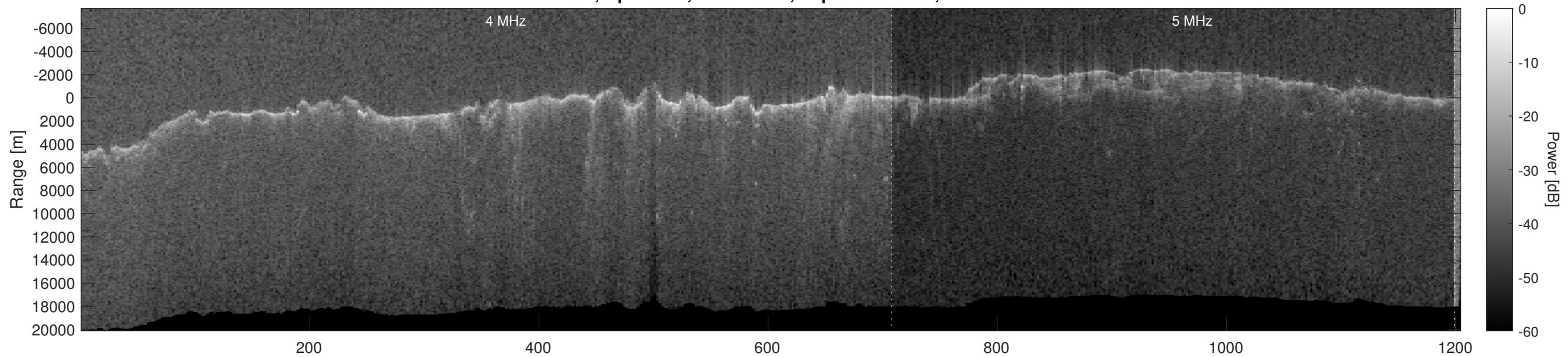
Orbit 4790, Optimized, No Window, Depth-Corrected, Channel 2
