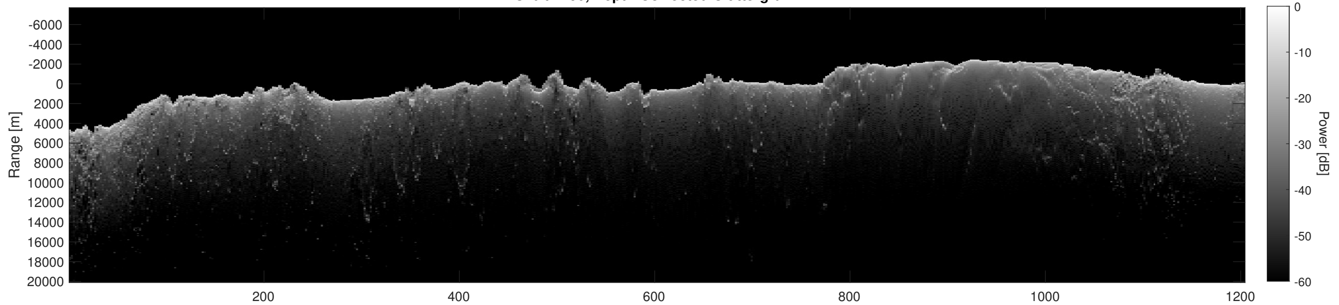
Orbit 4790, Depth-Corrected Cluttergram
