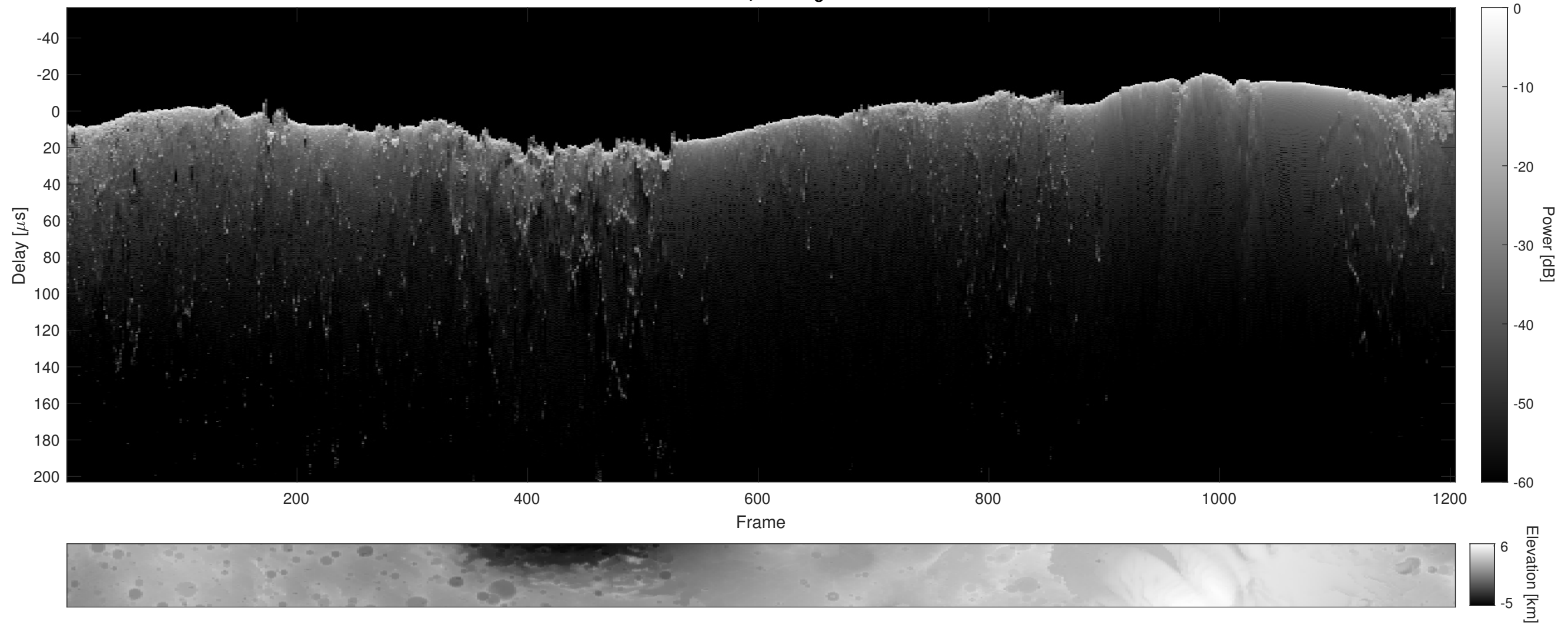
Orbit 4791, Cluttergram
