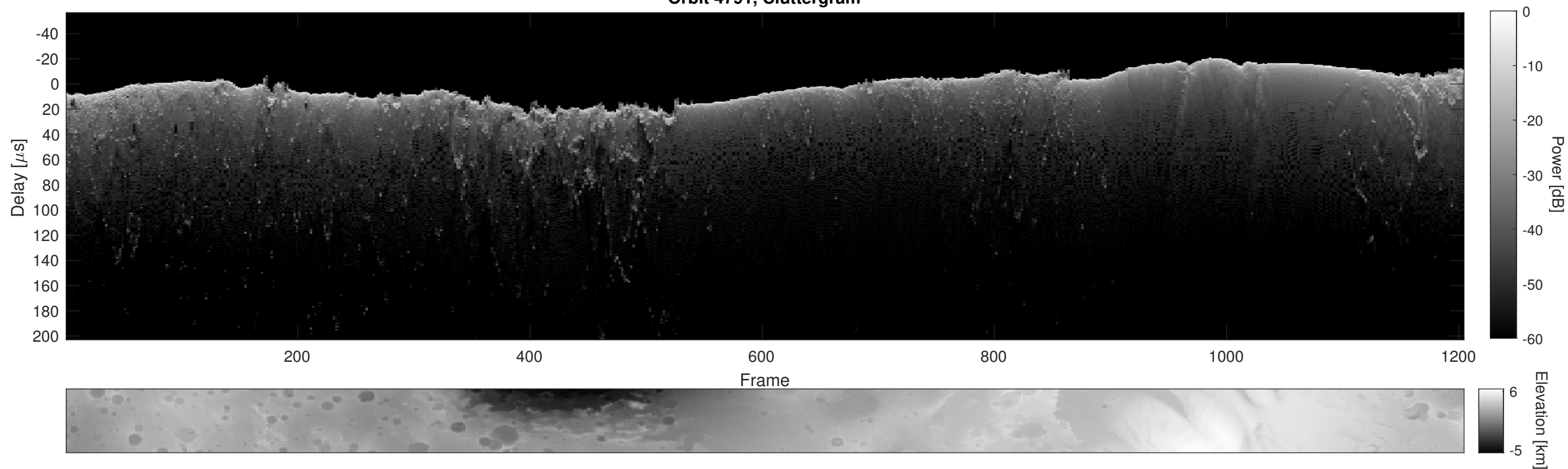
Orbit 4791, Cluttergram
