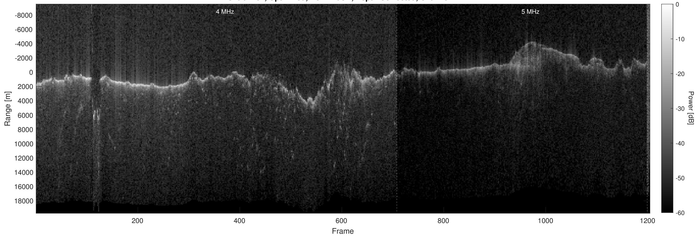
Orbit 4792, Optimized, No Window, Depth-Corrected, Channel 2
