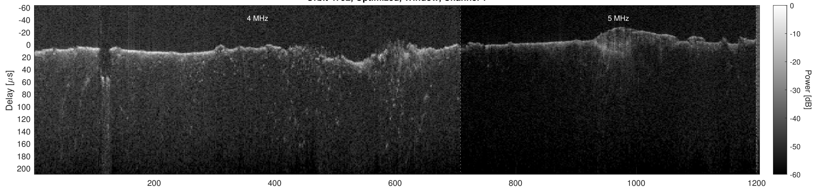
Orbit 4792, Optimized, Window, Channel 2
