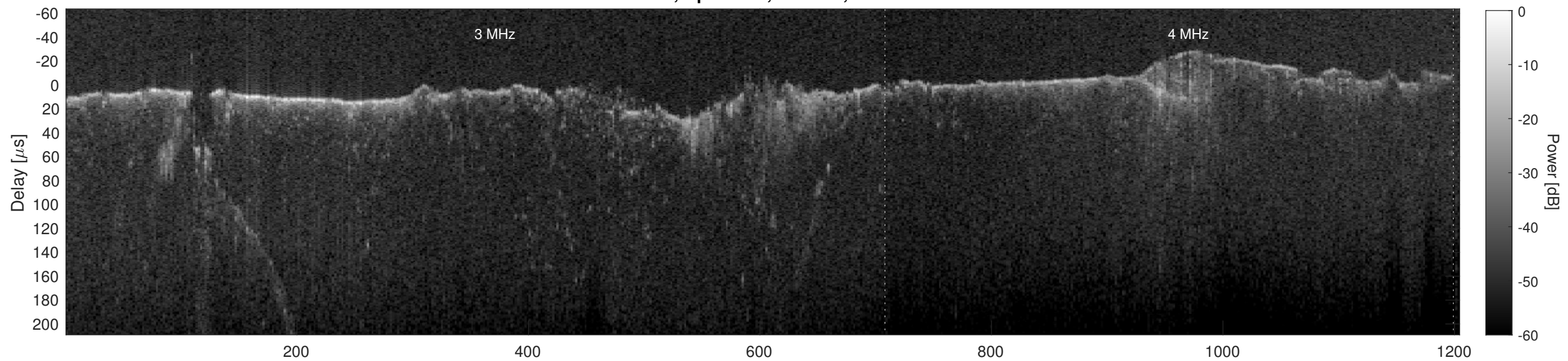
Orbit 4792, Cluttergram
