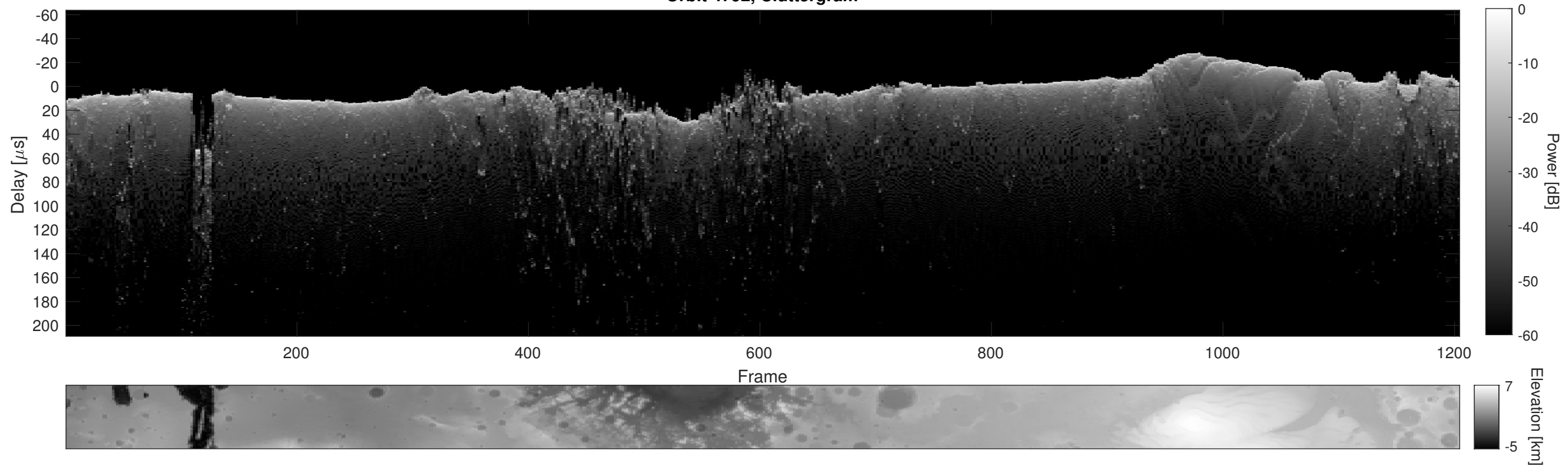
Orbit 4792, Cluttergram
