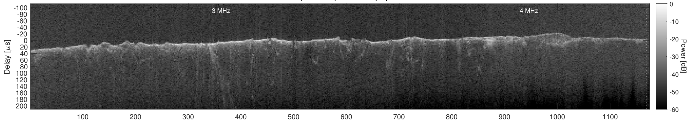
Orbit 4793, Cluttergram
