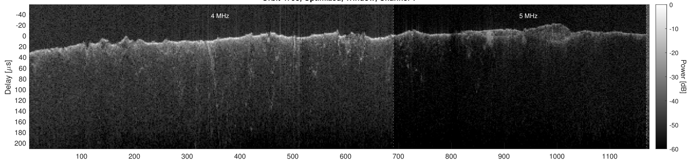
Orbit 4793, Optimized, Window, Channel 2
