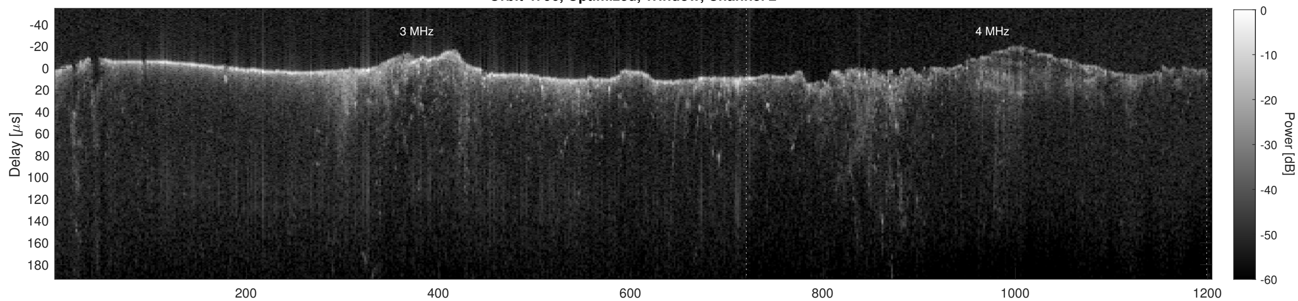
Orbit 4796, Cluttergram
