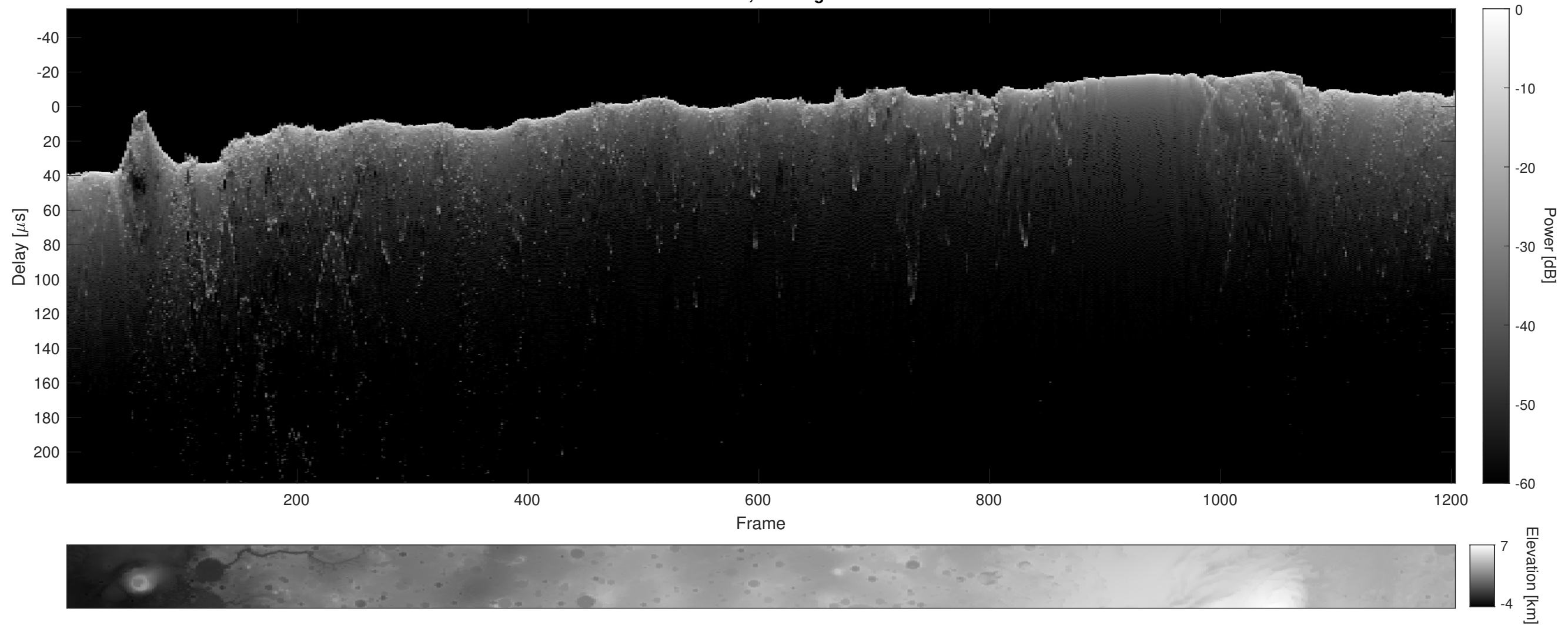
Orbit 4797, Cluttergram
