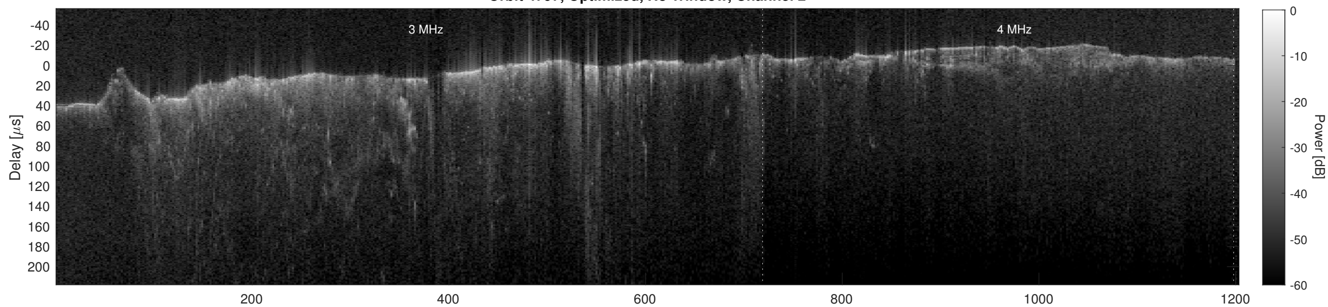
Orbit 4797, Cluttergram
