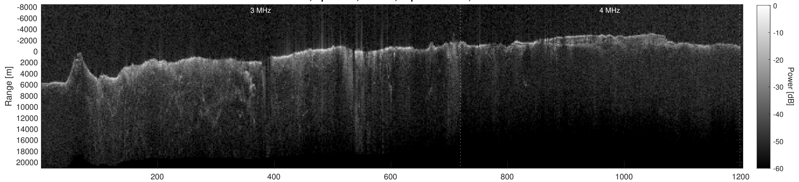
Orbit 4797, Depth-Corrected Cluttergram
