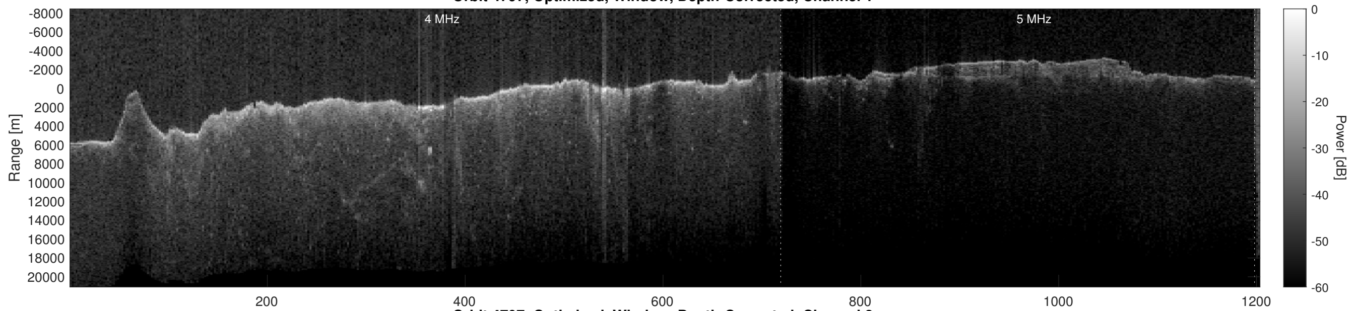
Orbit 4797, Optimized, Window, Depth-Corrected, Channel 2
