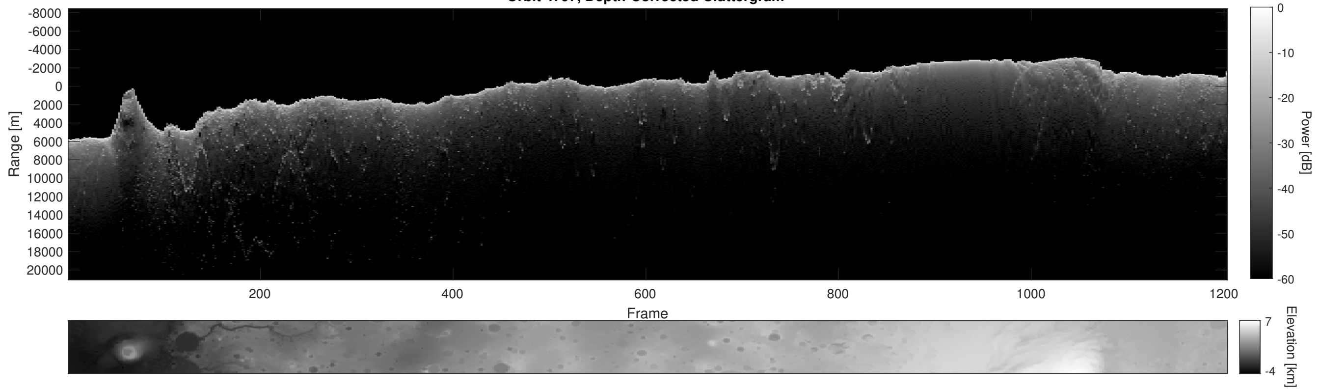
Orbit 4797, Depth-Corrected Cluttergram
